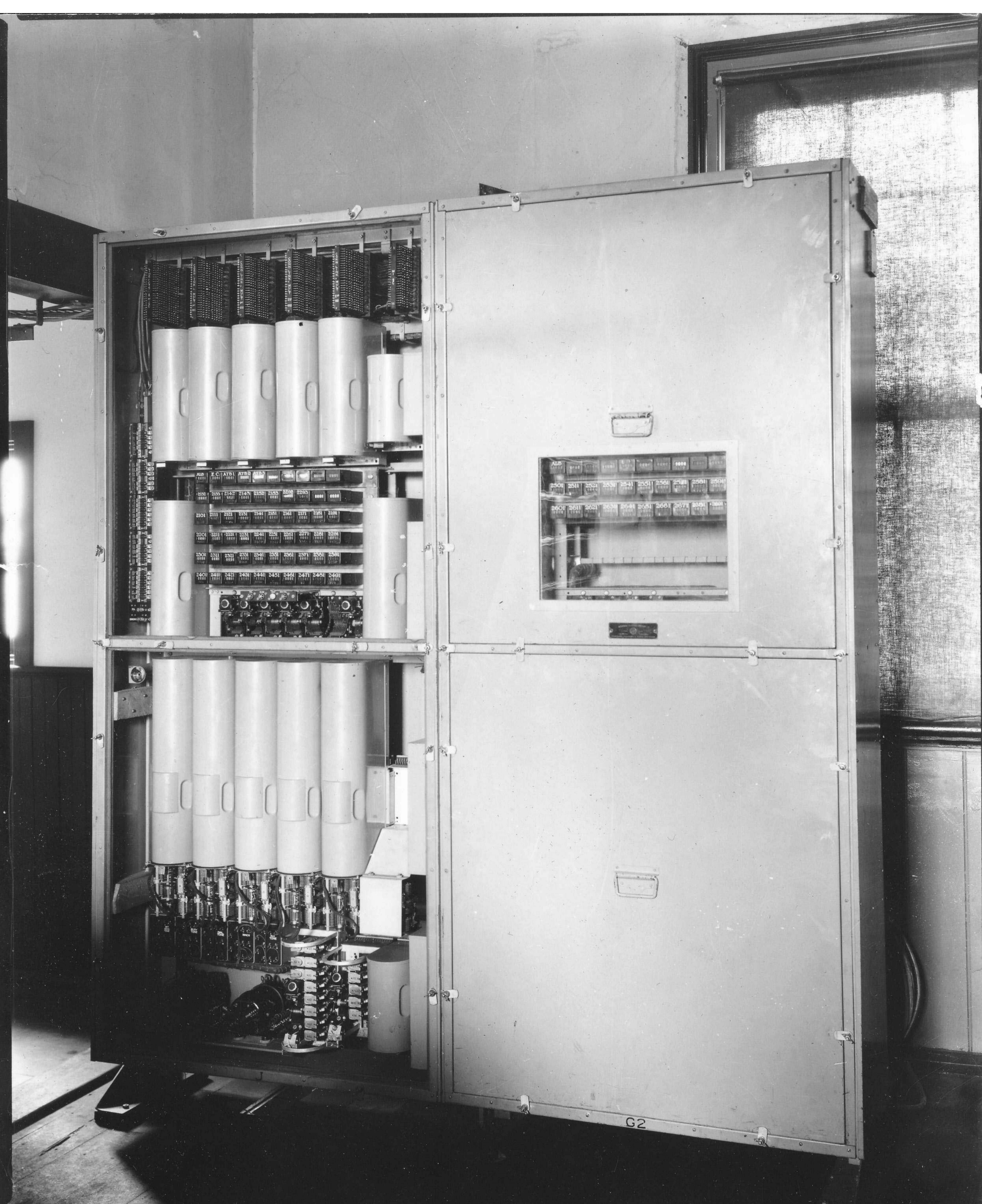
BRUNSWICK JUNCTION R.A.X. UNITS - Front view, one cover removed.
